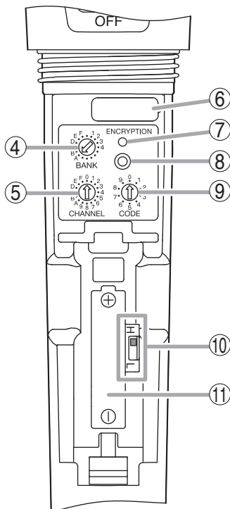
[Battery case internals – front]
