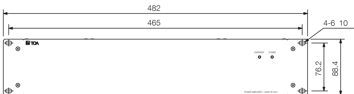
Front View
