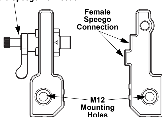
Bottom Male Bracket
