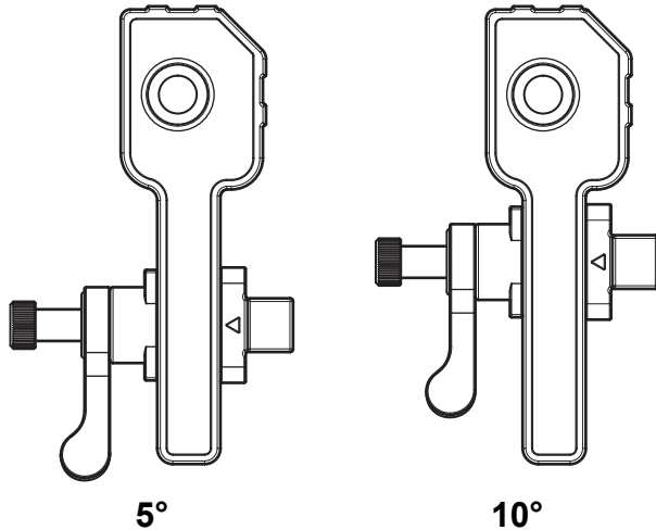
Top Male Bracket
