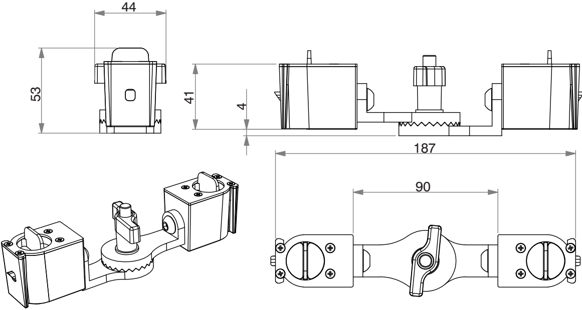
Pivot coupler (for interlocking two fixtures at an angle)
