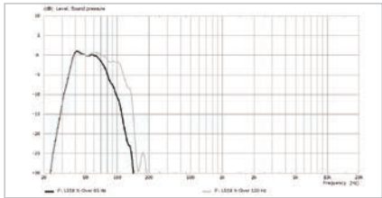
LS18 response
