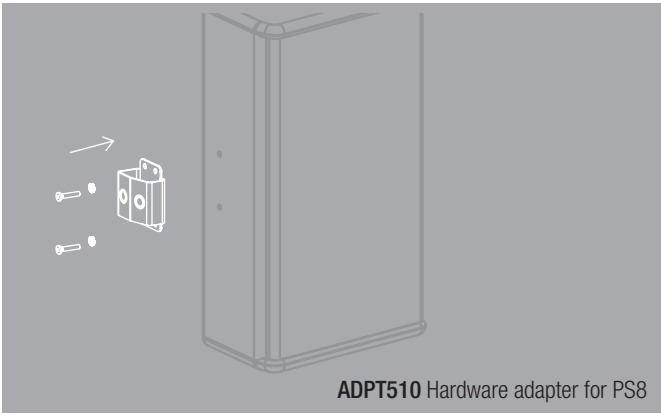
WS-10 Fixed hanging bracket for PS8 & PS10-R2 WS-15 Fixed hanging bracket for PS15-R2
