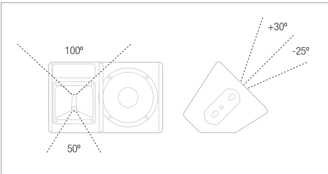
Stage monitor configuration
