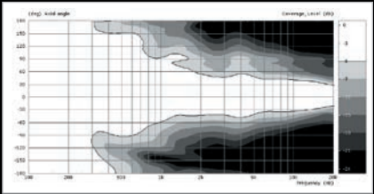
PS8 horizontal coverage, 0°
