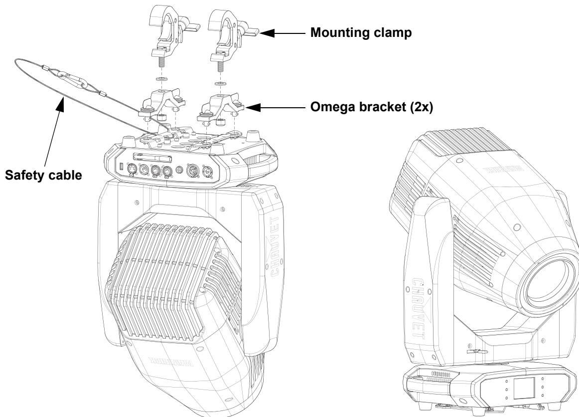
Overhead mounting
