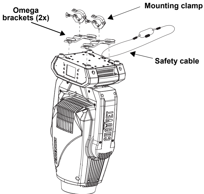
Overhead Mounting
