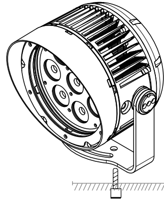
Floor Mounting
