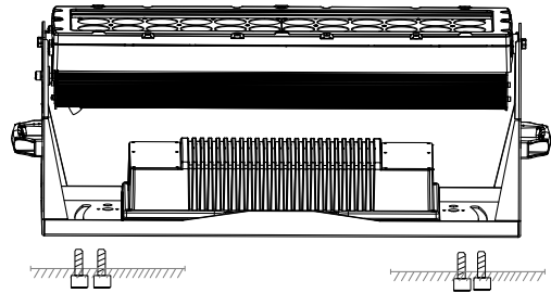
Floor Mounting
