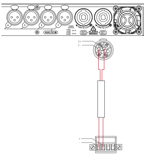
Figure 4.10: Bias Q5
