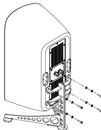
Figure 5.3: Bracket attachment
