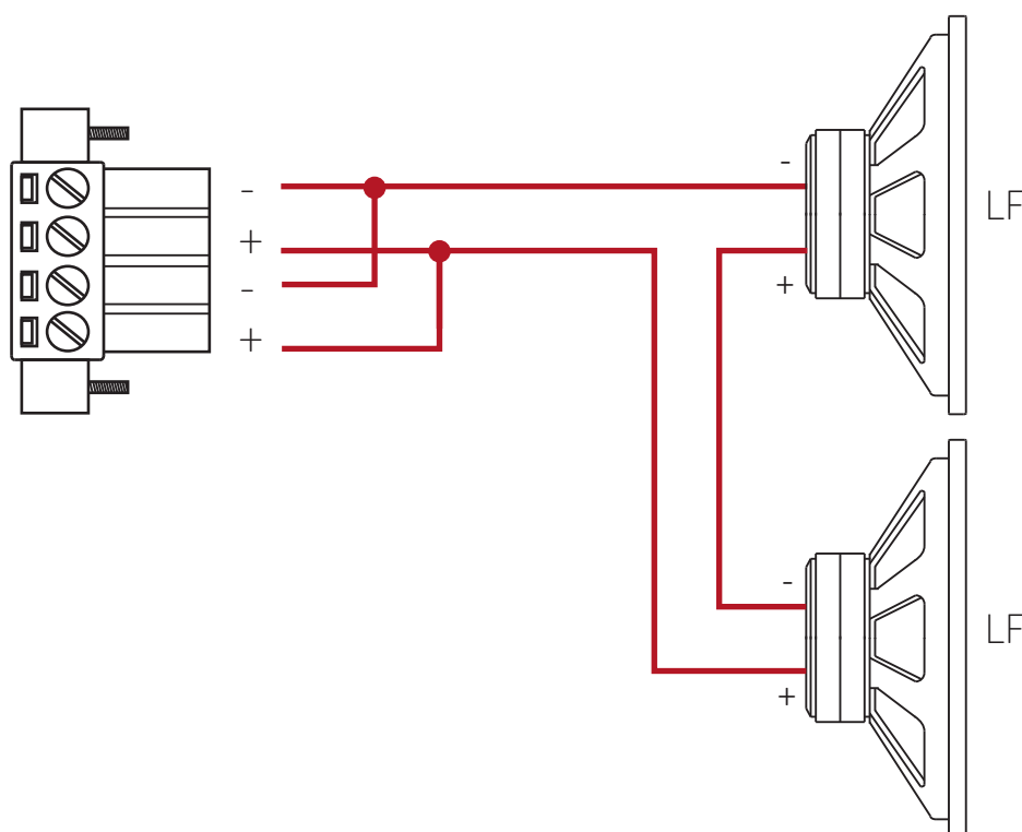
Figure 4.6: Cyclone 208 wiring diagram
