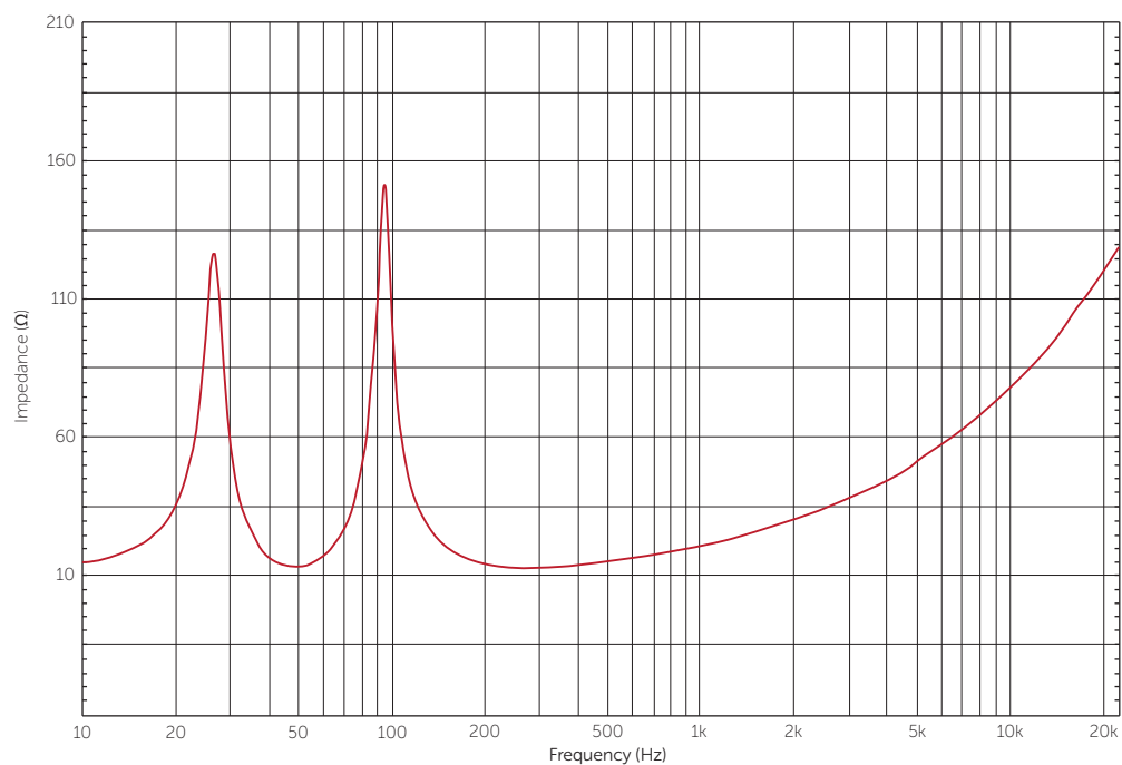
Figure 3.1: Impedance graph
