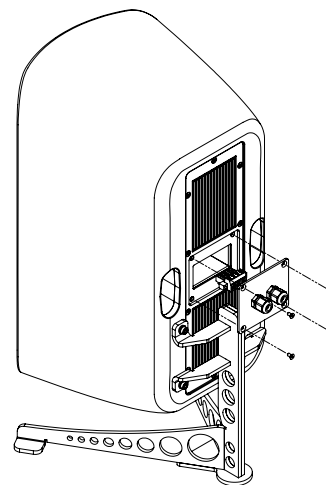
Figure 4.2: Connector plate removal
