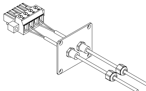
Figure 4.4: Cable connection
