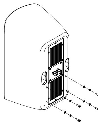
Figure 5.2: Bolt removal
