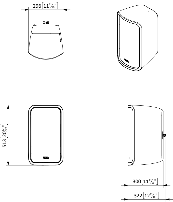
Figure 3.2: Dimensions
